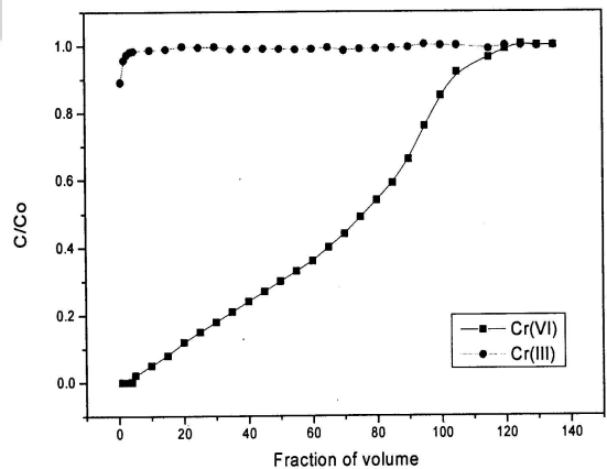
Fig. 8. Breakthrough curves of Cr(III) and Cr(VI) metal ions.
