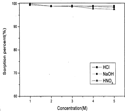
Fig. 2. Chemical stability of XAD-16-CTA chelating resin in acidic and basic solutions.
