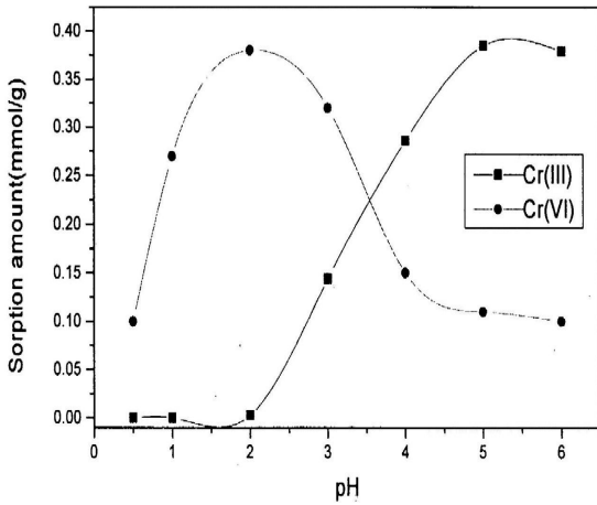
Fig. 3. Effect of pH on sorption of Cr(III) and Cr(VI) ion. Conc. of each metal ion : 50 ppm/50 mL XAD-16-CTA resin : 50 mg (100 ~ 200 mesh) Matrix : pH 2.0, 0.03 M KCl-HCl solution Shaking time : 24 hrs.
