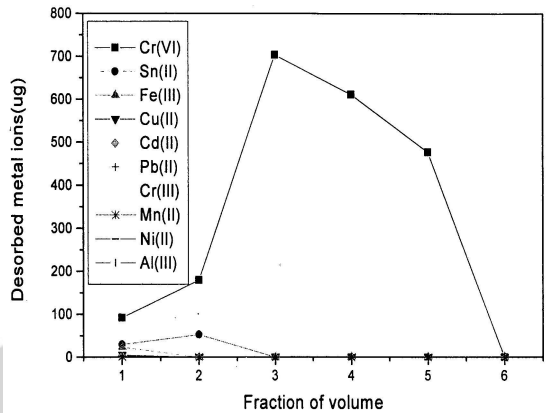
Fig. 10. Recovery of metal ions from artificial waste water solutions. XAD-16-CTA: 100 mg (100 ~ 200 mesh) Flow rate: 0.28 mL/min Fraction volume : 4 mL/fraction.
