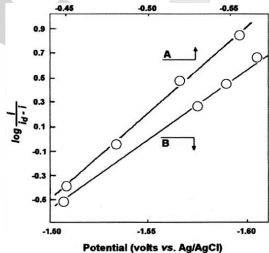
Fig. 3. A plot of \log i / (i - i) vs. potential from 1 \times 10^{-3} M ABMC polarograms.
