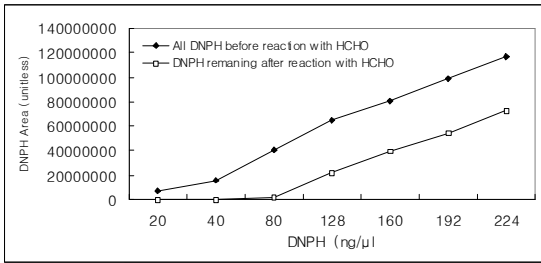
Fig. 3. A test to check for limiting role of DNPH in the formation of formaldehyde-DNPH derivatives. (Refer to Table 4 for the data used to draw this Fig. 3.
