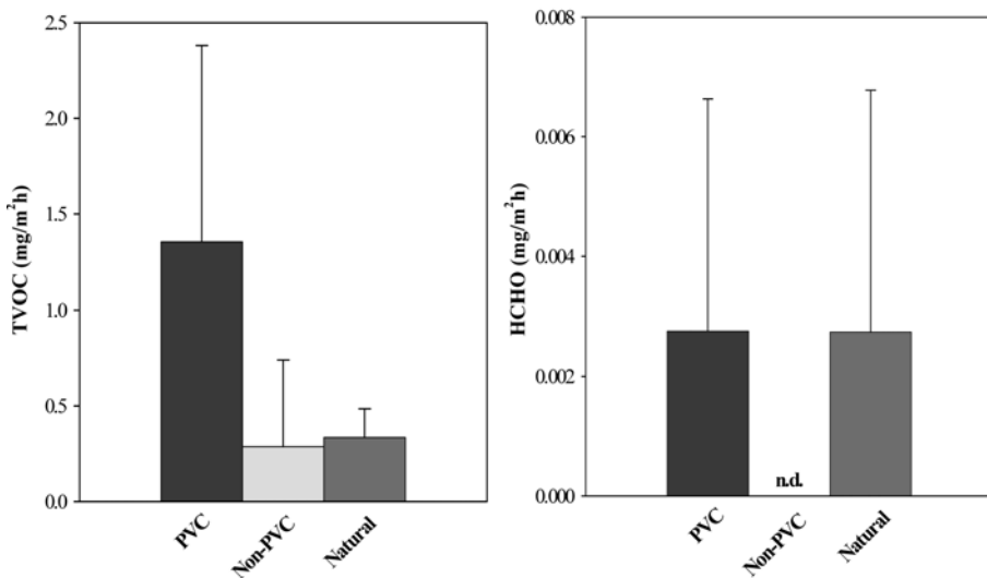
Fig. 4. Classificational comparison of TVOC and HCHO emission factor from wallpapers.
