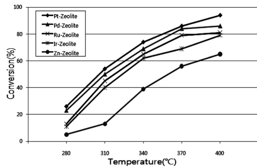
Fig. 10. Mixed PE, PP, and ABS conversion according to various catalysts.
