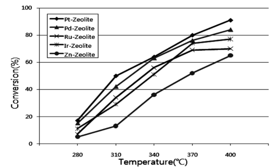
Fig. 9. ABS dissociation conversion according to various catalysts.
