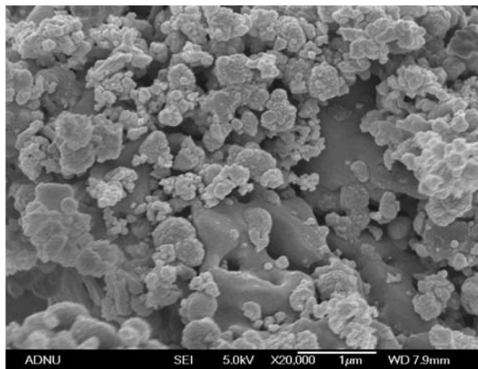
Fig. 4. SEM image of the Pt-Zeolite catalyst.
