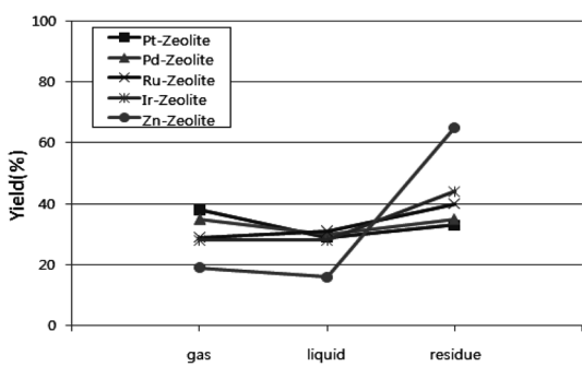
Fig. 11. Product distribution of PE at 340 °C according to various catalysts.
