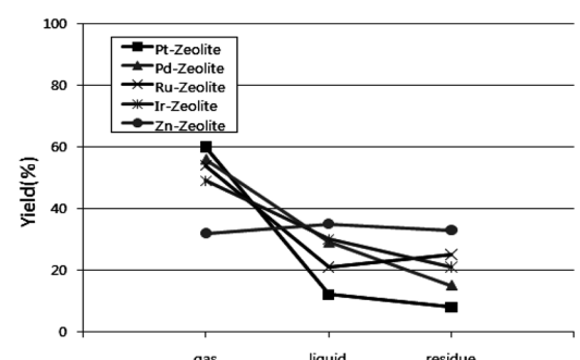
Fig. 12. Product distribution of PE at 400 °C according to various catalysts.
