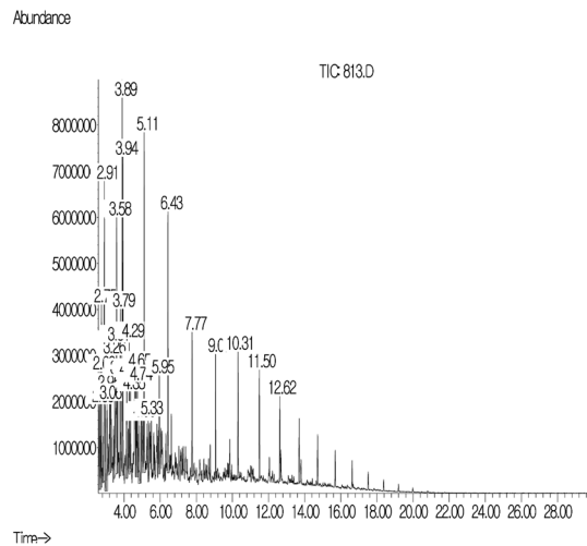
Fig. 16. GC/MS peaks of product distribution for PE catalytic dissociation at 400 °C.
