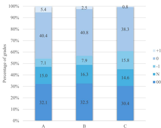
Fig. 3. Distribution of the percentage of grades received on comparing Ethanol-based BAC or CTAB post-treatment with nin(PE) development without post-treatment. A. Comparison between nin(PE) development without post-treatment and BAC or CTAB post-treatment within the same split fingerprint. B. Comparison before and after BAC or CTAB post-treatment within the same fingerprint. C. Comparison between nin(PE) development without post-treatment and BAC or CTAB post-treatment across several repeats
