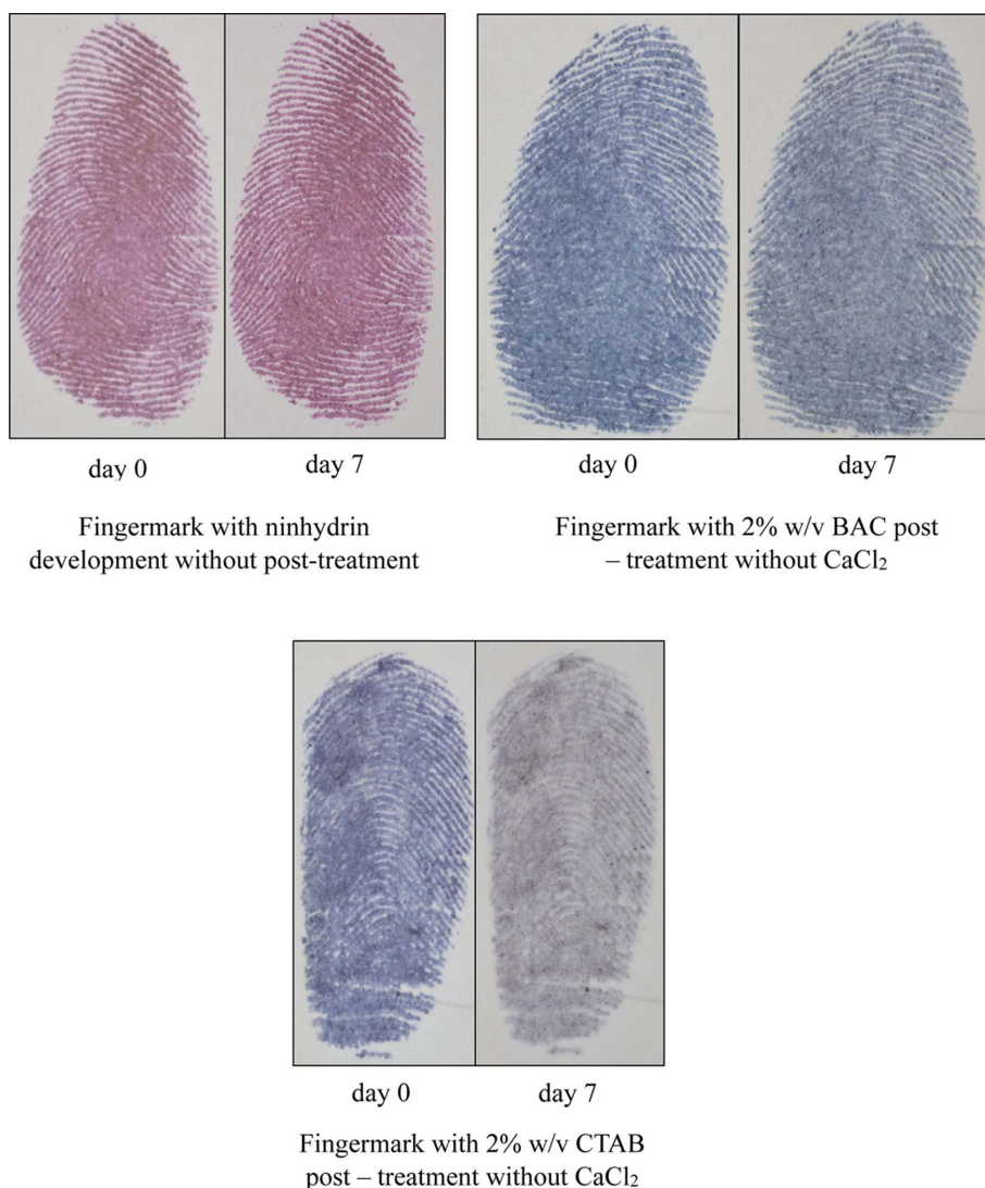
Fig. 2. Fading of fingerprints observed on day 7 after post-treatment with 2 % w/v Ethanol-based BAC and 2 % w/v Ethanol-based CTAB compared to ninhydrin development without post-treatment.
