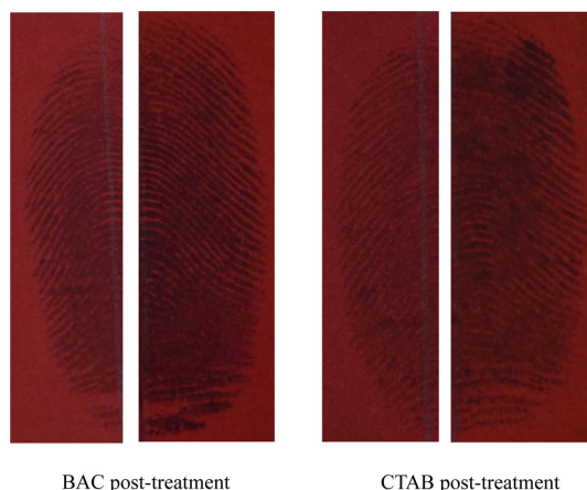
Fig. 4. Comparison of ninhydrin-developed fingerprints on crimson paper before (left halves) and after (right halves) 2 % w/v ethanol-based BAC/CTAB post-treatment.
