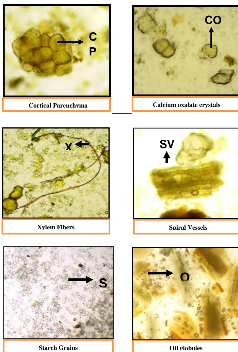
Fig.5 Powder microscopy
