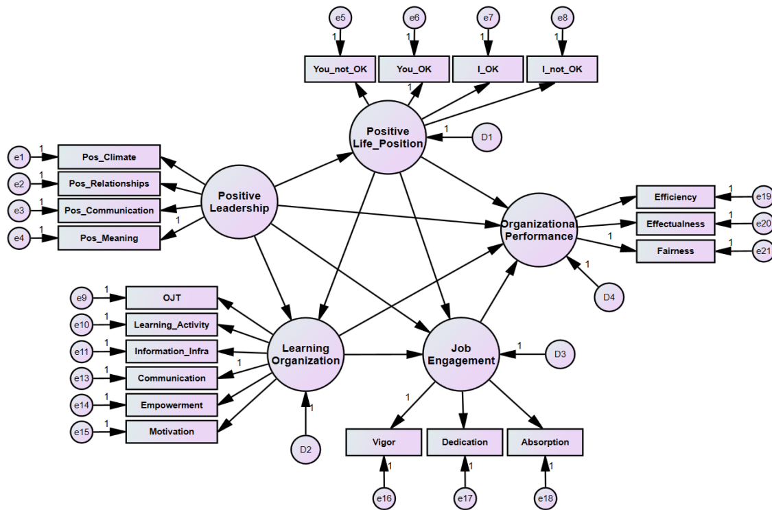
&lt;Figure 5&gt; Statistical Models
