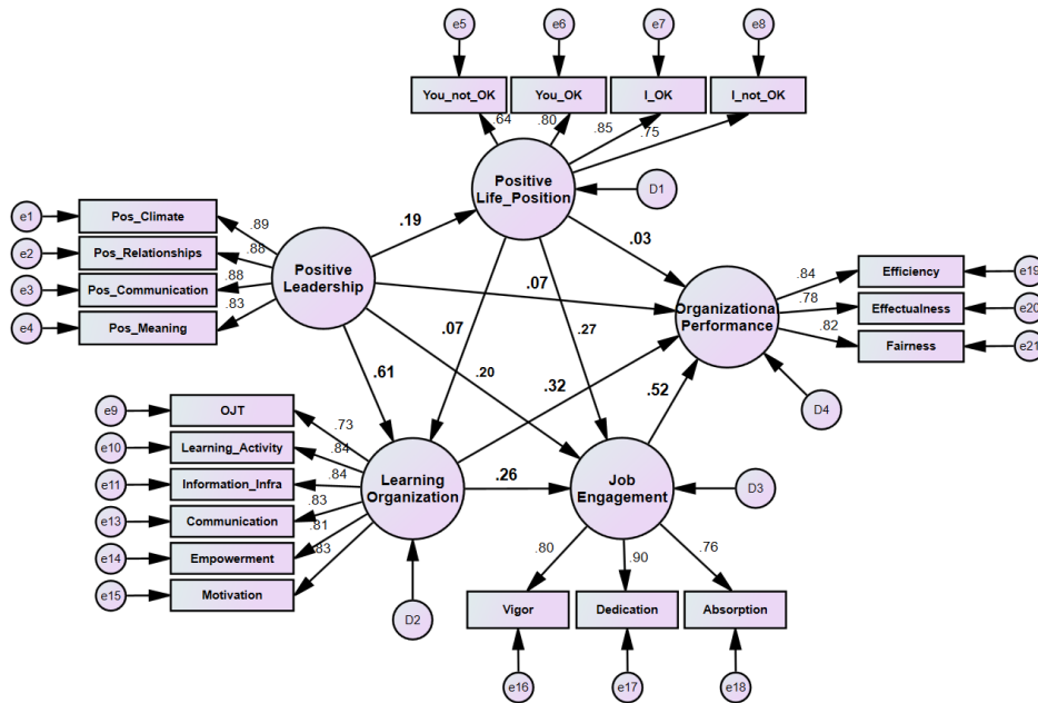
<Figure 7> Early Structural Regressive Model(Standardized Coefficients)
