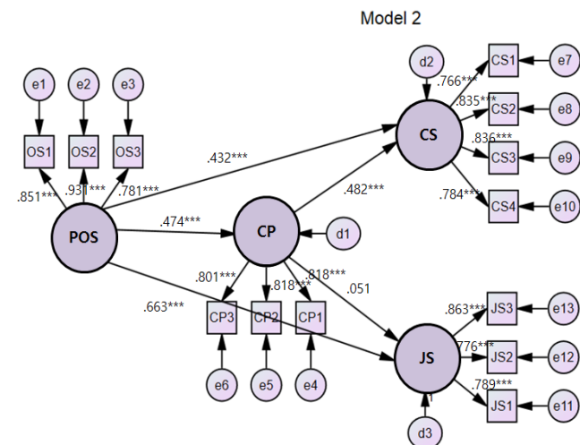
<Figure 2> Final Model (Model 2) with Standardized Path Coefficients
