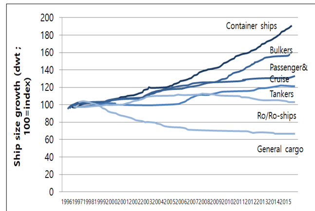
<Figure 2> Ship Size of Ship Types 1996-2015
