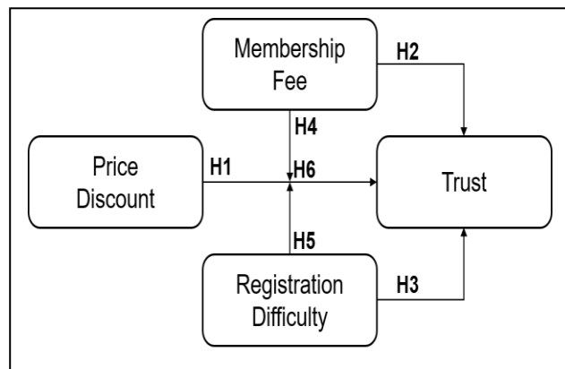
Figure 1: Research Model
