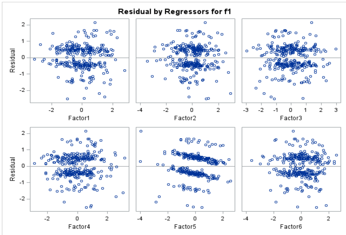
Figure 3: Fit Plots
