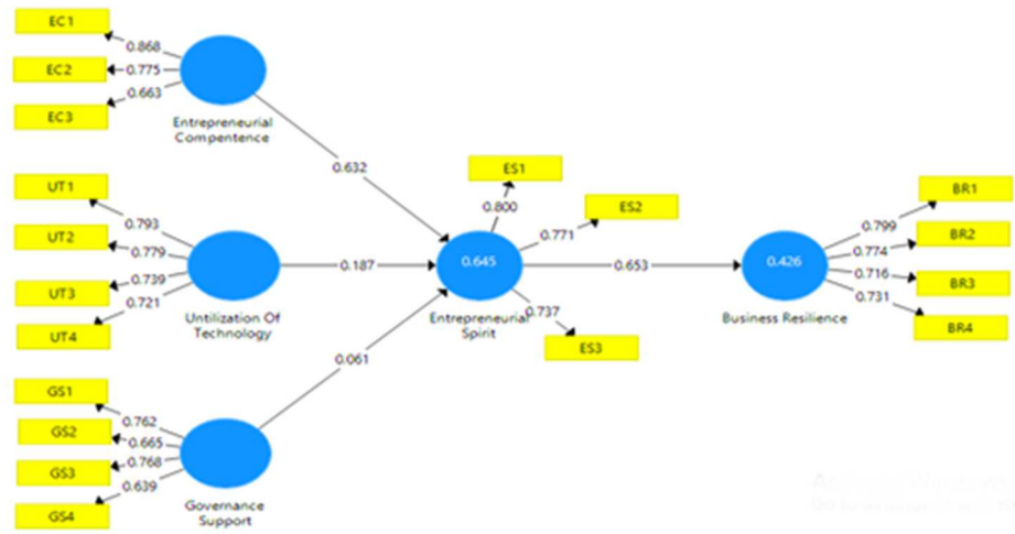
Figure 2: PLS Analysis
