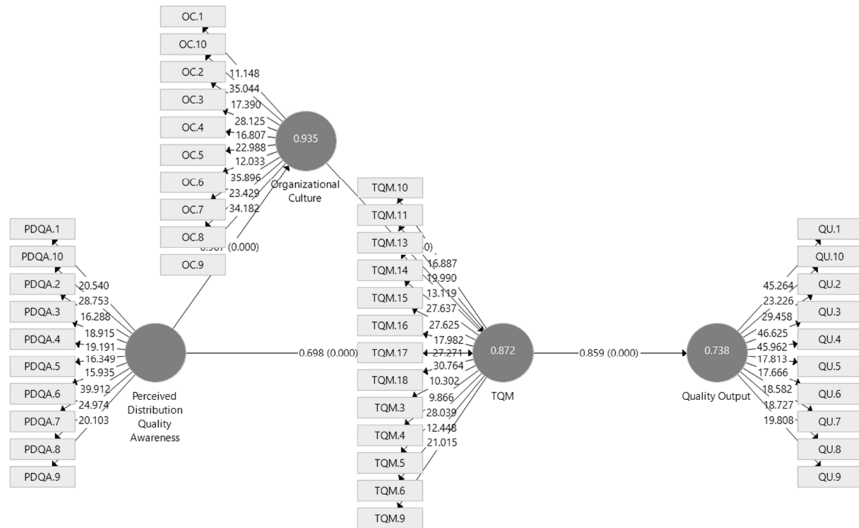
Figure 1: SEM-PLS Result
