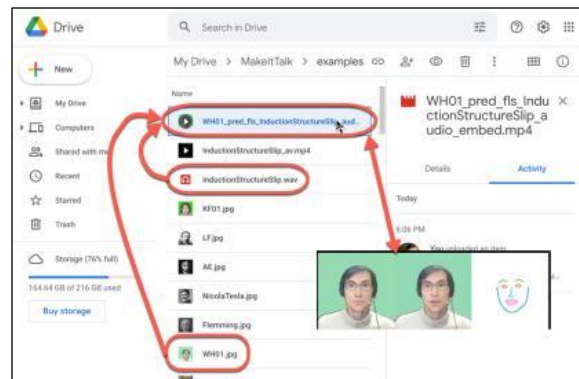
Figure 8: Run MakeItTalk
