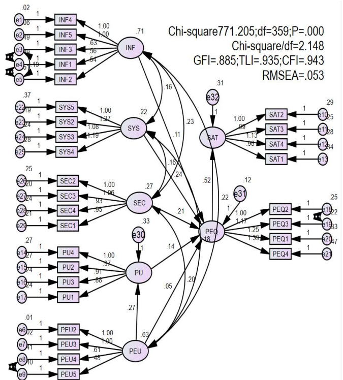
Figure 3: Test Research Hypotheses Using SEM
