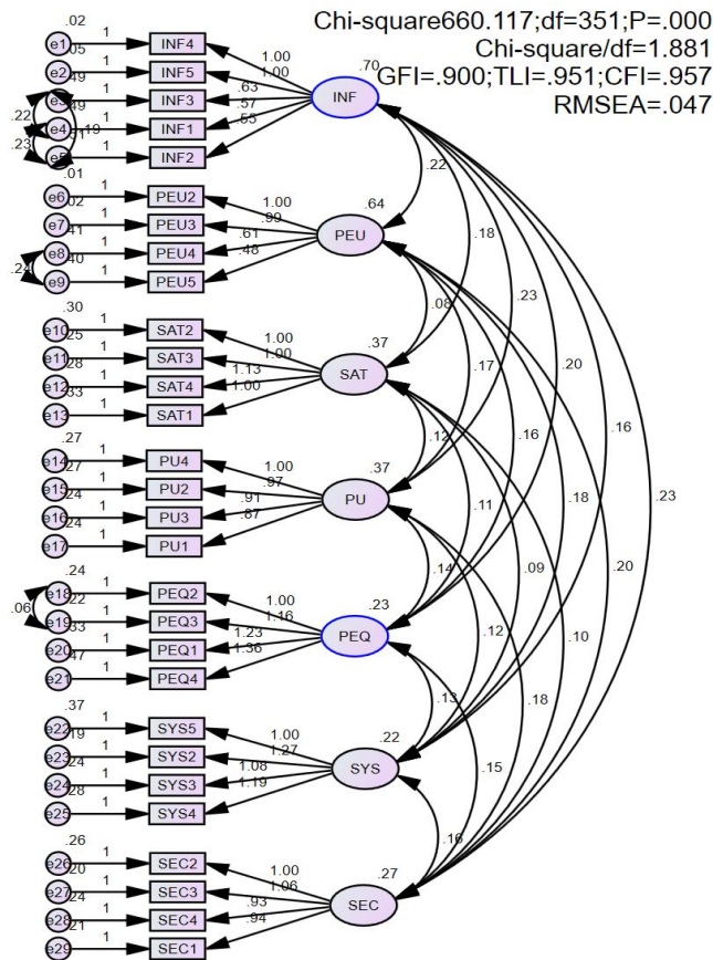
Figure 2: CFA Model
