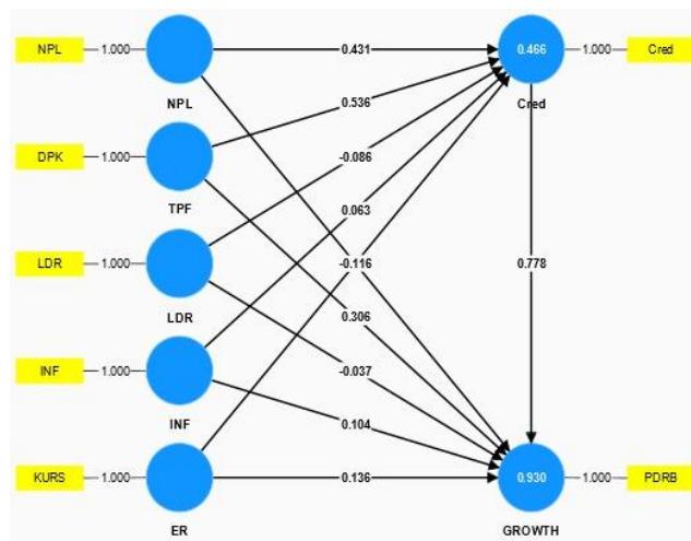
Figure 2: Algorithm Analysis
