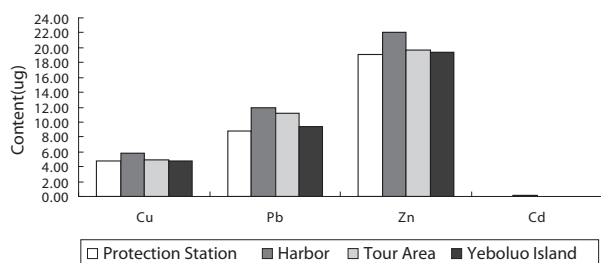
Fig. 2. Comparison of heavy metal content in different soil samples.
