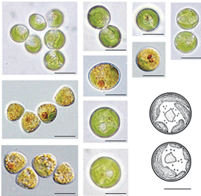
Fig. 7. Microscopic photographs and illustrations of Eustigmator polyphem (Pitschmann) Hibberd found in Hongcheon-river of Gangwon-do from December 2011 to June 2012. Scale bars, 10 \mu m.
