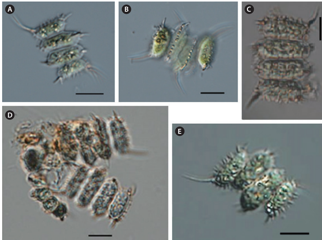
Fig. 7. Scenedesmus lefevrei . Scale bars, 10 µm.
