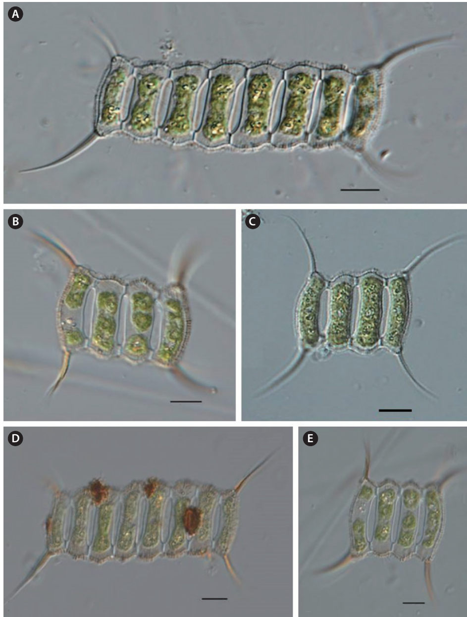
Fig. 14. Scenedesmus oahuensis var. clathratus . Scale bars, 10 \mu\text{m} .
