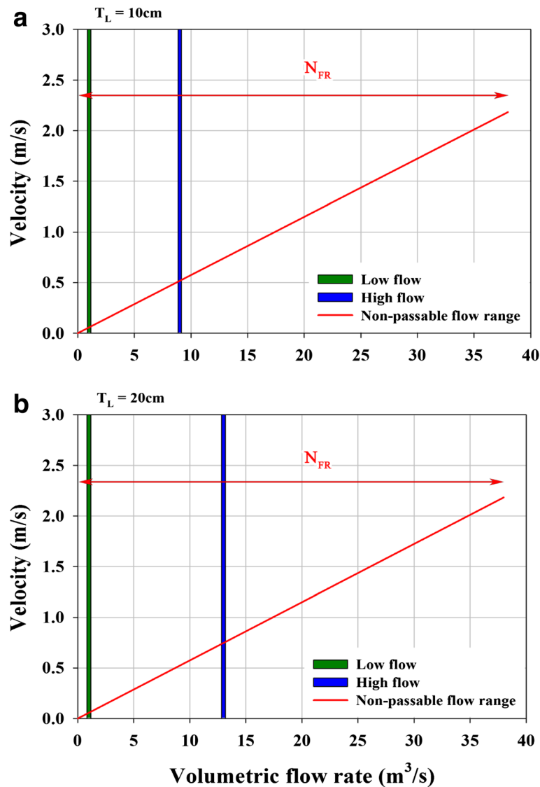
Fig. 5 Passable ( P_{FR} ) or non-passable ( N_{FR} ) flow range of the calculated inflow rates for juvenile/young largemouth bass based on size of individuals (total length (cm), T_L )
