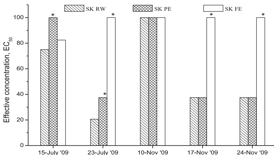
Fig. 3 Seasonal variations of the EC 50 s of SK STP effluents. Asterisks indicate significant difference with respect to raw wastewater samples
