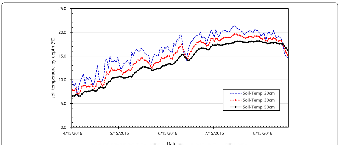
Fig. 10 The patterns of mean daily soil temperature at different depth during a growing season on Mt. Hallasan in 2016
