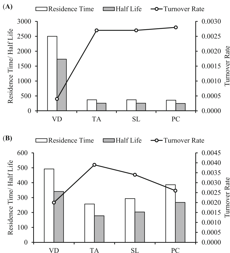
Fig. 4 Residence time, half-life, and turnover rate of four species. a Dry season. b Wet season. VD, Vitex doniana ; TA, Terminalia avicennioides ; SL, Sarcocephalus latifolius ; PC, Parinari curatellifolia
