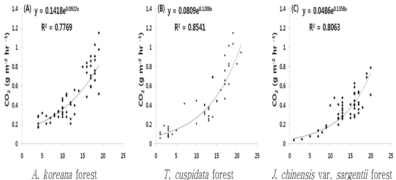
Fig. 2 Relationship between soil respiration (g m -2 h -1 ) and soil temperature (°C) at 5-cm depth in three subalpine forest ecosystems (a: A. koreana forest, b: T. cuspidata forest, c: J. chinensis var. sargentii forest)
