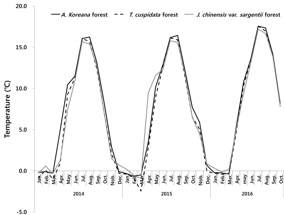
Fig. 1 Monthly fluctuation in temperature of soil at 5-cm depth in the forest ecosystems in the subalpine zone, Jeju Island, over multiple years. The three lines represent the temperature of soil at 5-cm depth in each forest (black solid line, A. koreana forest; black dotted line, T. cuspidata forest; gray solid line, J. chinensis var. sargentii forest)
