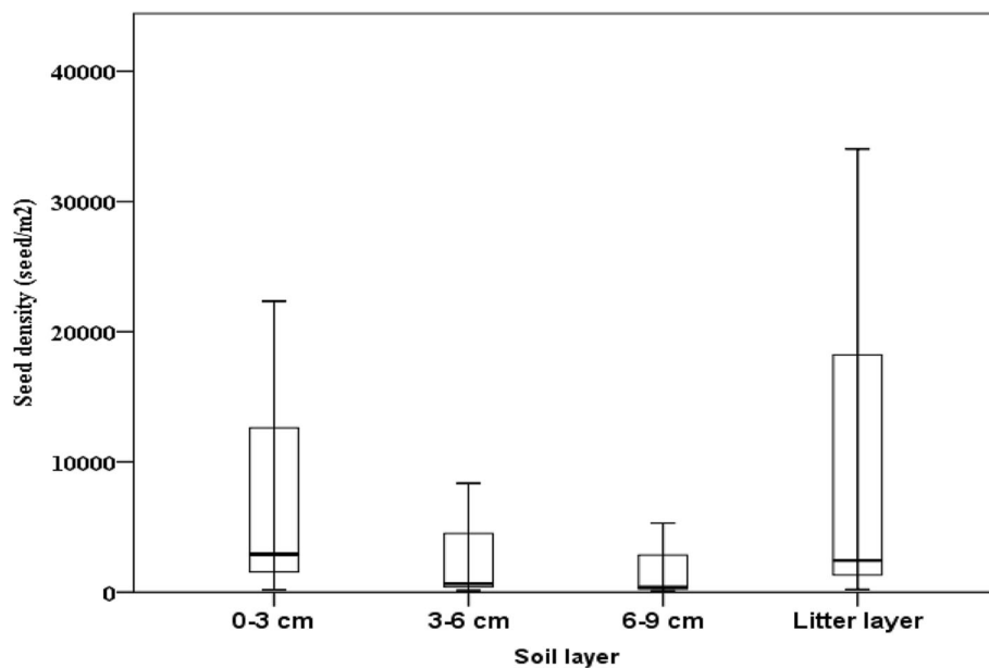
Fig. 3 The vertical distribution of density of soil seed bank
