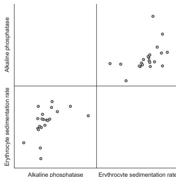
Fig. 4. Scatterplot matrix that shows a moderate degree of positive correlation ( r=0.474 , P<0.05 ) between the changes of preoperative and postoperative erythrocyte sedimentation rate (ESR) and alkaline phosphatase (ALP) in all patients. The changes in ALP were occurred in tandem with the changes in ESR.
