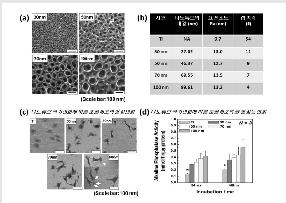
그림 2. (a) SEM micrographs of self-aligned titania nanotubes with different diameters. (b) Table with the average pore size distribution, roughness (Ra), and surface contact angle of titanium and 30~100nm titania nanotube surfaces. (c) SEM micrographs of osteoblast cultured on different sized nanotube surfaces. (d) Bone building functionality represented by alkaline phosphatase activity of osteoblasts cultured on the different sized nanotube surfaces.
