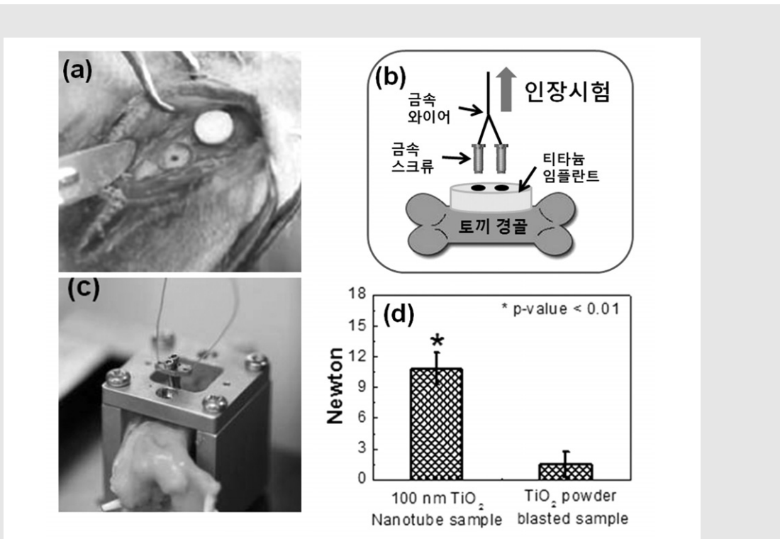
그림 3. Rabbit implant test process and result, (a) Sample positioning on rabbit tibia, (b) mechanical testing arrangement, (c) test fixture for tensile loading, and (d) comparative rabbit implant strengths by tensile pull out test.
