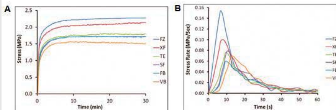
그림 2 A Comparison of the shrinkage stress development as a function of time for the five measured bulk-fill composites and control. B. Shrinkage stress rate development in time within the 60 seconds from composite irradiation of the investigated materials. FZ: Filtek Z250, XF: x-tra fil, TE: Tetric EvoCeram bulk fill SF: Surefil SDR flow, FB: Experimental flowable, VB: Venus Bulk Fill Polymerization Shrinkage Stress Kinetics and Related Properties of Bulk-fill Resin Composites. Operative Dentistry 39(4) 374-382
