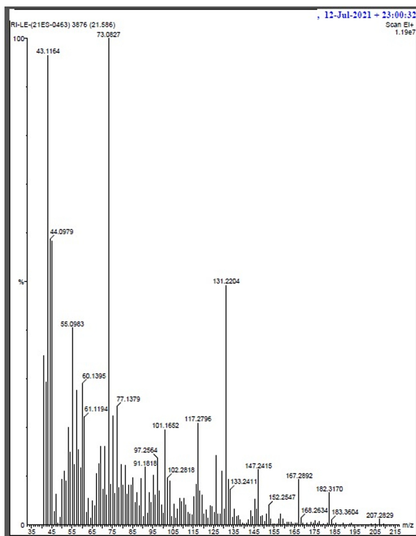
Fig. 1. Mass spectra of the methanolic leaf extract of Ricinus communis major compound (Pentanoic,2-(aminooxy)-).
